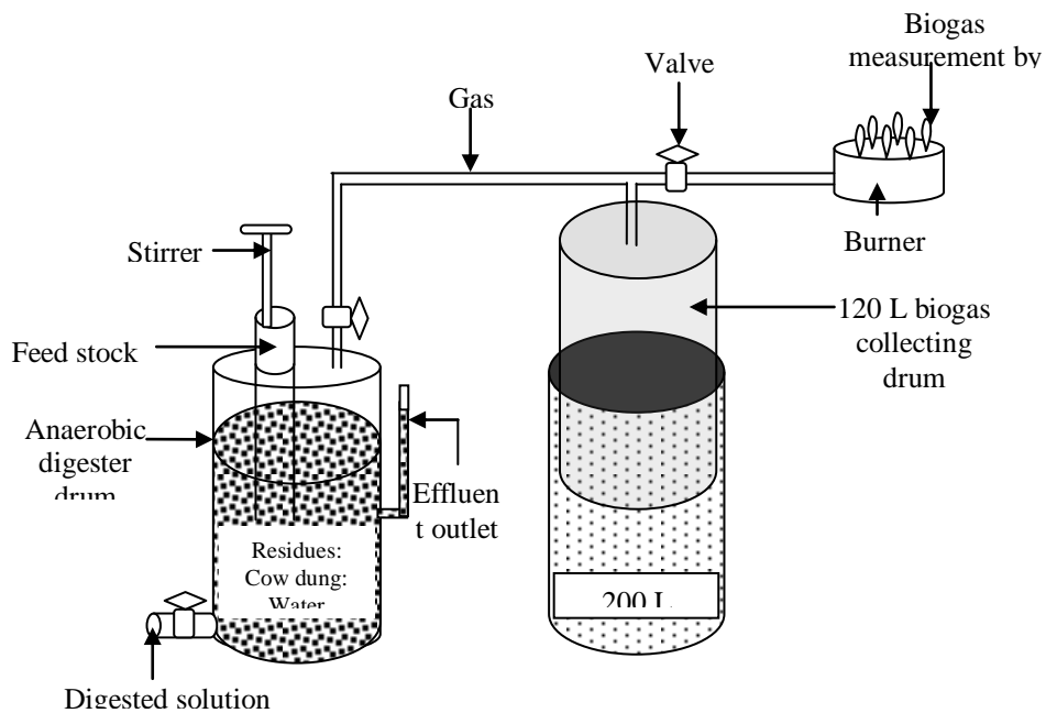
Fig.1. Diagram of a floating drum digester
